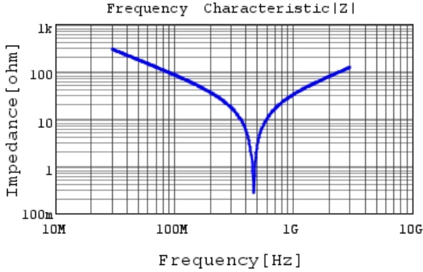
RCE5C2A180J0M1H03A |Z| DC0V, 25degC
