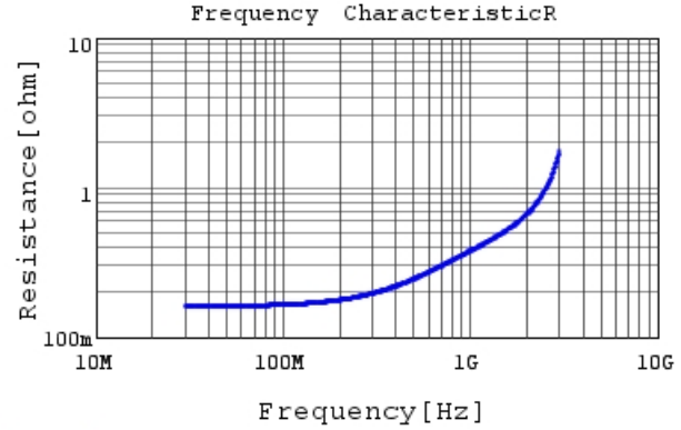
RCE5C2A180J0M1H03A R DC0V, 25degC
