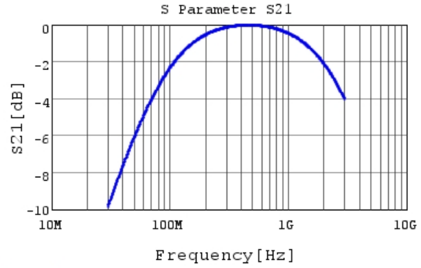
RCE5C2A180J0M1H03A S21 DCOV, 25degC
