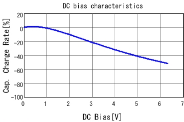
GRM32EE70J476KE20 C-DC bias capchange, 25.0degC, A
