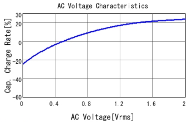
GRM32EE70J476KE20 C-AC Voltage capchange, DCOV, 25
