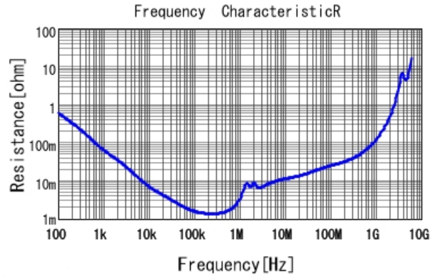
GRM32EE70J476KE20 R DCOV, 25degC
