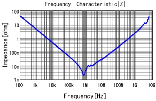
GRM32EE70J476KE20 |Z| DCOV, 25degC
