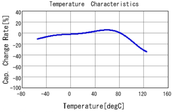
GRM32EE70J476KE20 C-Temp. capchange, DC0.0V, AC0.5
