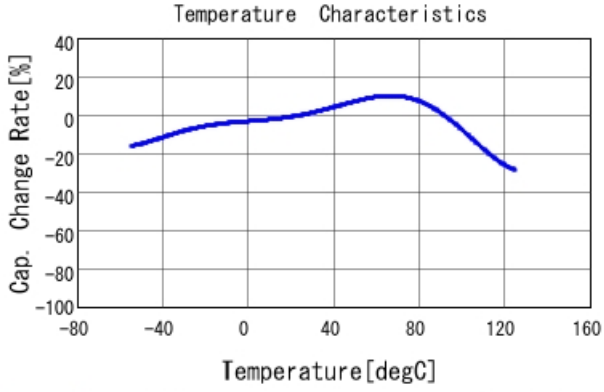
GRM32ED70J476KE20 C-Temp. capchange, DC0.0V, AC0.3
