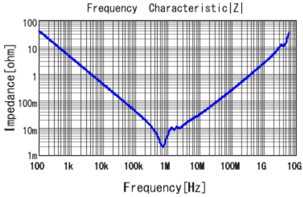
GRM32ED70J476KE20 |Z| DCOV, 25degC
