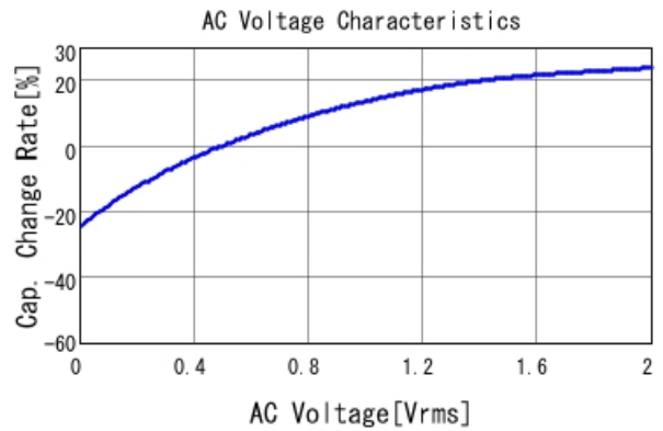
GRM32ED70J476KE20 C-AC Voltage capchange, DCOV, 25
