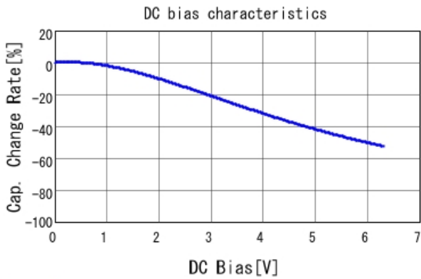
GRM32ED70J476KE20 C-DC bias capchange, 25.0degC, A
