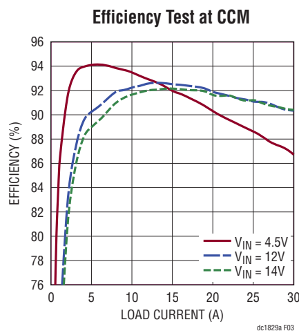
Figure 3. Efficiency vs Load Current
