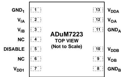
Figure 3. Pin Configuration
