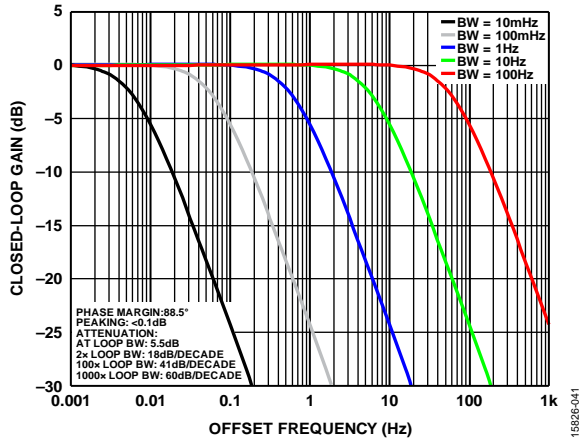
Figure 21. DPLL Closed-Loop Transfer Function Nominal Phase Margin Loop Filter Setting
