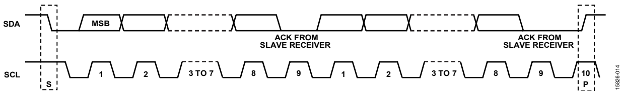
Figure 61. Acknowledge Bit
