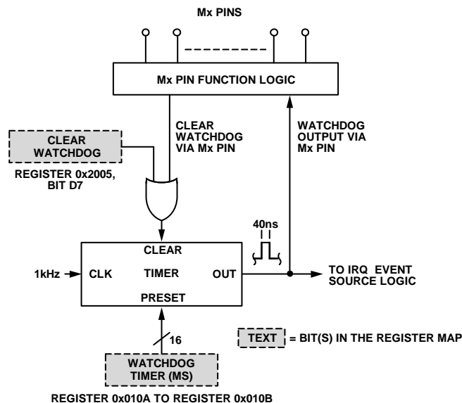
Figure 48. Watchdog Timer
