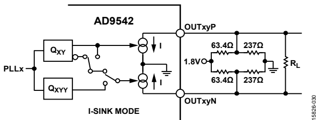
Figure 35. LVDS-Compatible Output, 1.2 V Common-Mode, Thevenin Bias Network ( I = 7.5\text{ mA} ; I = 15\text{ mA} With Extra 100 Ω Termination, R_L )
