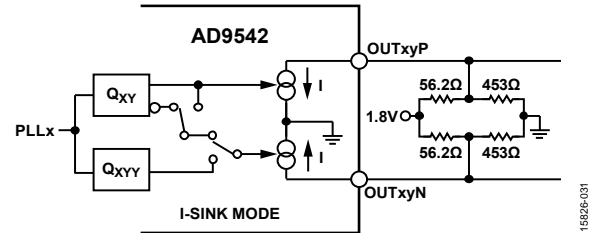
Figure 36. 2.5 V LVPECL or Double Amplitude LVDS-Compatible Boost Output, 1.5 V p-p , 1.24 V Common-Mode ( I = 15\text{ mA} )
