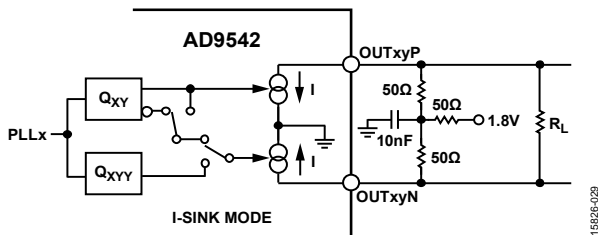
Figure 34. LVDS-Compatible Output, 1.24 V Common-Mode, T Network ( I = 7.5\text{ mA} ; I = 15\text{ mA} With Extra 100 Ω Termination, R_L )
