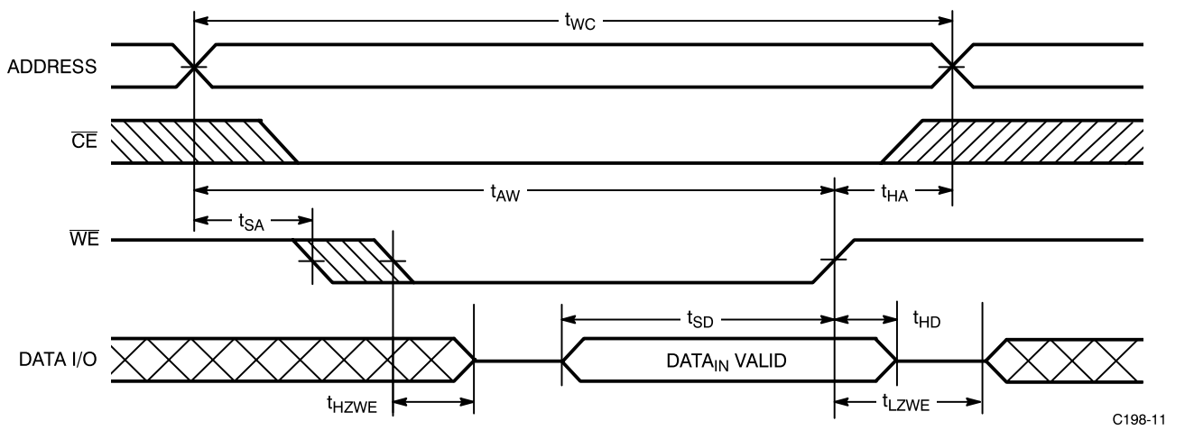
Write Cycle No. 3 ( \overline{WE} Controlled, \overline{OE} LOW)[25, 30]
