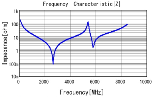
GQM2195G2H9R0CB12 |Z| DCOV, 25degC
