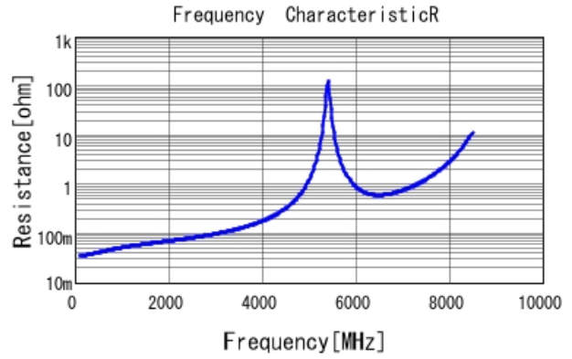
GQM2195G2H9R0CB12 R DCOV, 25degC
