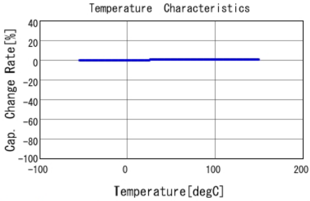
GQM2195G2H9R0CB12 C-Temp. capchange, DCOV, AC1Vrms
