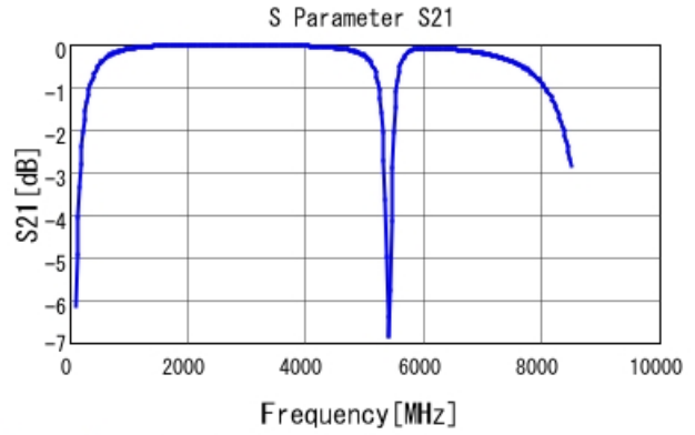
GQM2195G2H9R0CB12 S21 DCOV, 25degC
