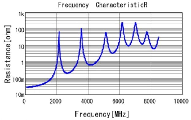
GQM22M5C2H560JB01 R DCOV, 25degC
