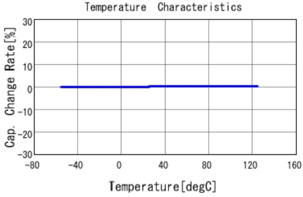
GQM22M5C2H560JB01 C-Temp. capchange, DCOV, AC1Vrms
