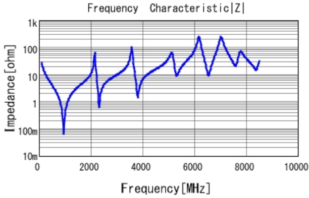
GQM22M5C2H560JB01 |Z| DCOV, 25degC
