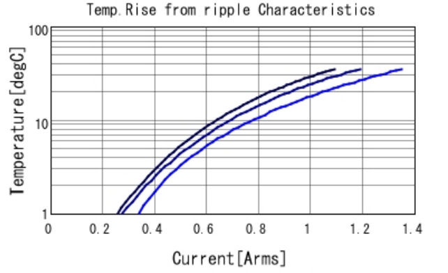
GQM22M5C2H560JB01 Temp. rise — 200MHz — 500
