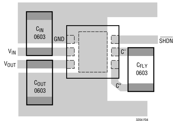
Figure 4. Recommended Layout
