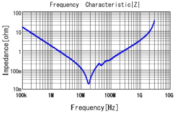
GRJ55DR73A104KWJ1 |Z| DCOV, 25degC
