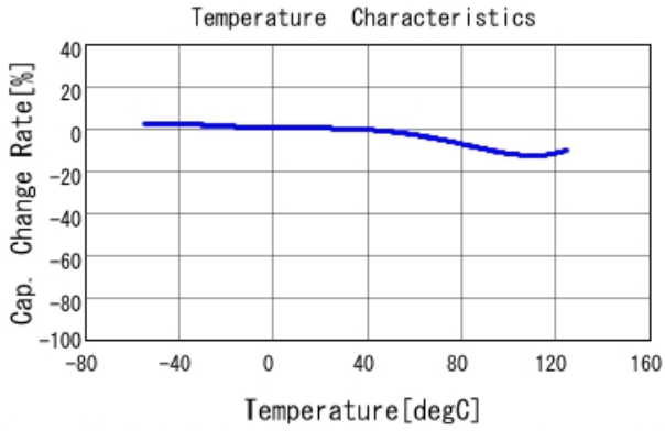
GRJ55DR73A104KWJ1 C-Temp. capchange, DCOV, AC1Vrms
