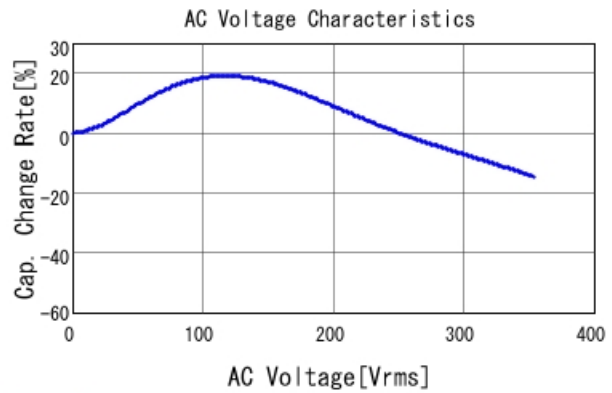
GRJ55DR73A104KWJ1 C-AC Voltage capchange, DCOV, 25
