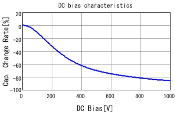
GRJ55DR73A104KWJ1 C-DC bias capchange, 25.0degC, A
