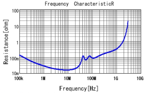
GRJ55DR73A104KWJ1 R DCOV, 25degC
