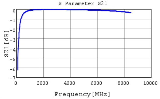
GRM0335C2A8R9WA01 S21 DCOV, 25degC
