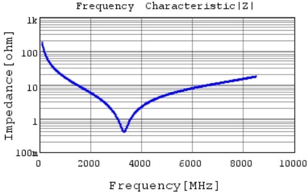
GRM0335C2A8R9WA01 |Z| DC0V, 25degC
