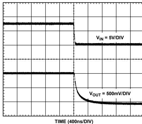
Figure 6. Turn-Off Time
