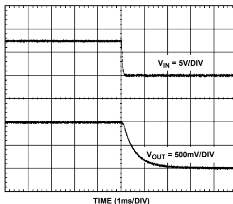
Figure 7. Turn-Off Time with 1 \mu F Input Capacitor
