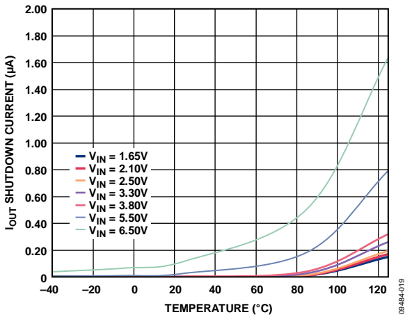
Figure 19. I_{OU2} Shutdown Current vs. Temperature, V_{OUT} = 0V
