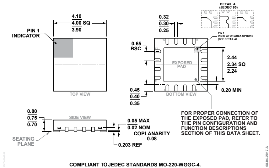
COMPLIANT TO JEDEC STANDARDS MO-220-WGGC-4. Figure 26. 16-Lead Lead Frame Chip Scale Package [LFCSP] 4 mm × 4 mm Body and 0.75 mm Package Height (CP-16-39) Dimensions shown in millimeters
