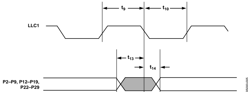
Figure 5. Pixel Port SDR Timing (CP Core)
