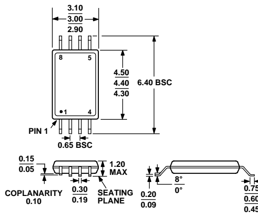
COMPLIANT TO JEDEC STANDARDS MO-153-AA Figure 17. 8-Lead Thin Shrink Small Outline Package [TSSOP] (RU-8)
