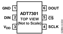
Figure 4. SOT-23
