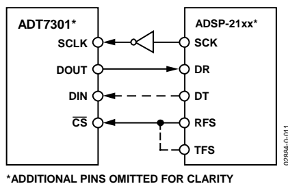
Figure 17. ADT7301 to ADSP-21xx Interface
