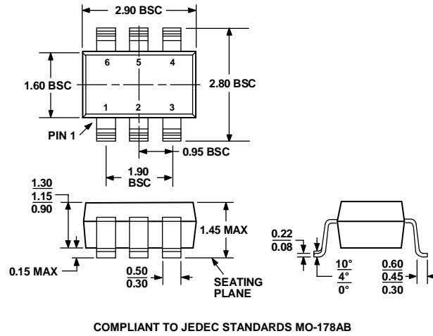
Figure 18. 6-Lead Small Outline Transistor Package [SOT-23] (RJ-6) Dimensions shown in millimeters
