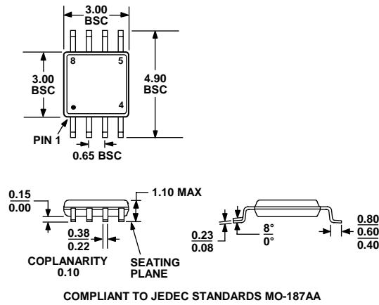
Figure 19. 8-Lead Mini Small Outline Package [MSOP] (RM-8) Dimensions shown in millimeters
