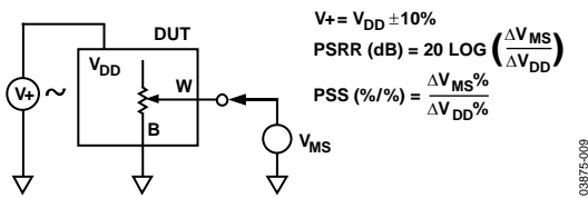
Figure 22. Test Circuit for Power Supply Sensitivity (PSS, PSRR)
