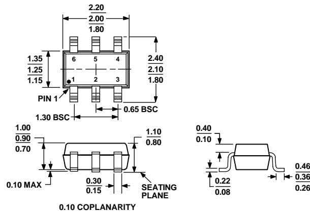
Figure 37. 6-Lead Thin Shrink Small Outline Transistor Package [SC70] (KS-6) Dimensions shown in millimeters
