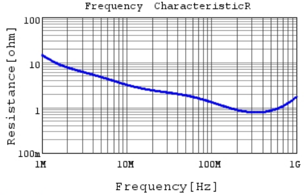
DE1B3RA331KA4BH01F R DC0V, 20degC
