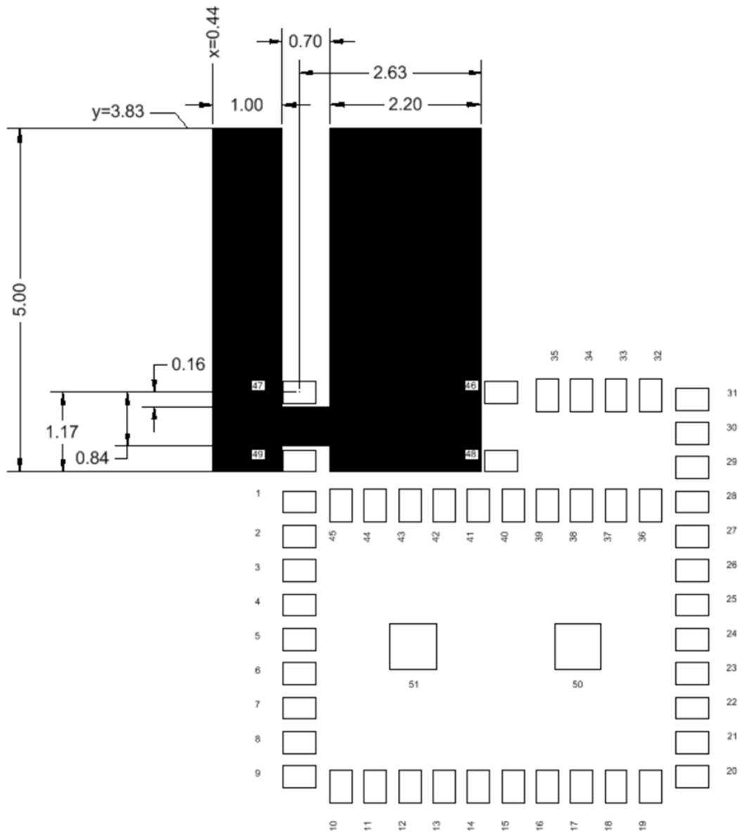
Figure 7.2. BGX13S Recommended Antenna Clearance
