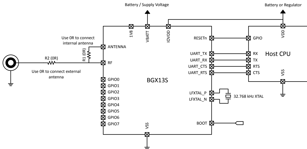
Figure 3.1. Typical Connections for BGX13S
