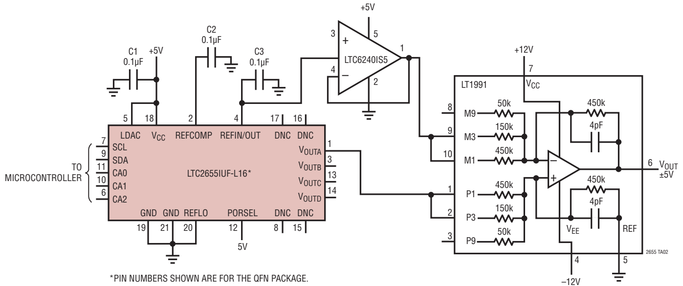
±5V Bipolar Output DAC
