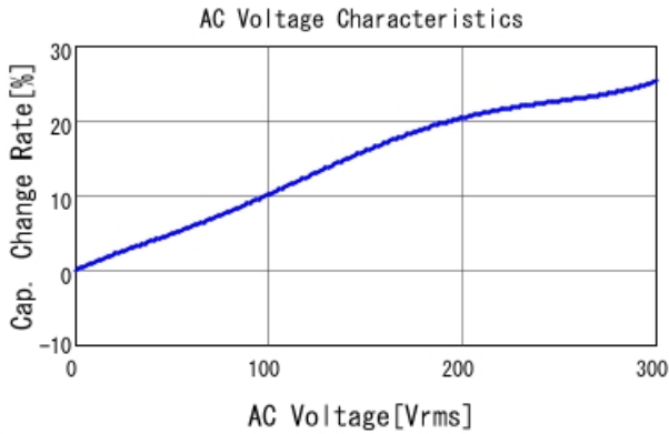
DE2B3SA221KA3BX02F C-AC Voltage capchange, DCOV, 2
