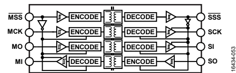
Figure 67. iCoupler Gating
