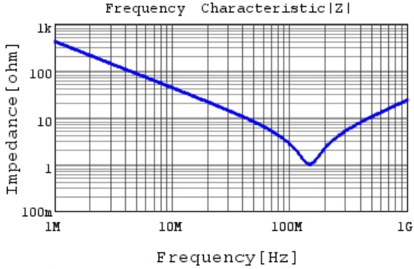
DK1B3EA471K86RAH01 |Z| DCOV, 20degC
