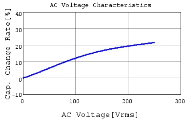
DK1B3EA471K86RAH01 C-AC Voltage capchange, I
