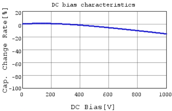
DK1B3EA471K86RAH01 C-DC bias capchange, 20.0
