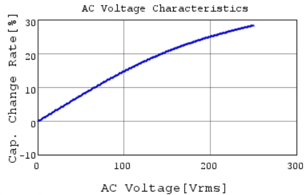
DE2B3SA681KA3BT02F C-AC Voltage capchange, I
