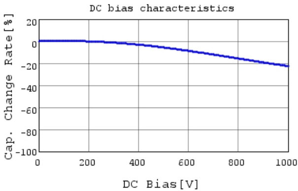
DE2B3SA681KA3BT02F C-DC bias capchange, 20.0
