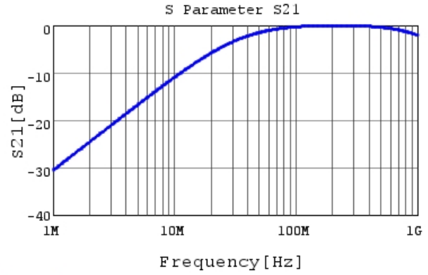
DE11XRA470KN4AH01F S21 DCOV, 20degC
