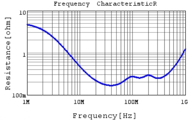
DE11XRA470KN4AH01F R DCOV, 20degC
