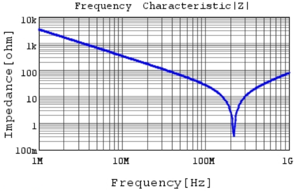
DE11XRA470KN4AH01F |Z| DCOV, 20degC
