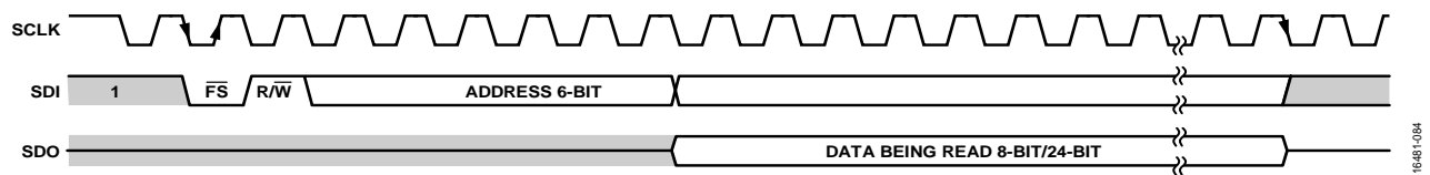
Figure 88. 3-Wire SPI Read Frame ( \overline{\text{CS}} = 0 )
