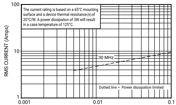
CURRENT RATING VS CAPACITANCE ATC SERIES 200, CASE B
