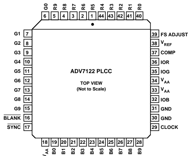
PLCC (P-44A) Package
