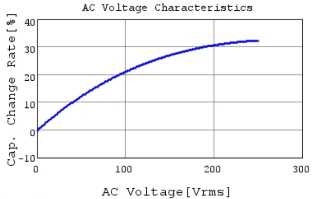
DE2E3KY152MB2BM01F C-AC Voltage capchange, I
