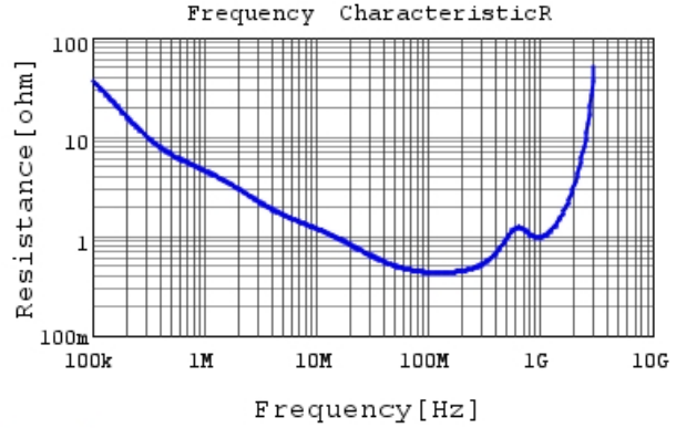
DE2E3KY152MB2BM01F R DC0V, 20degC
