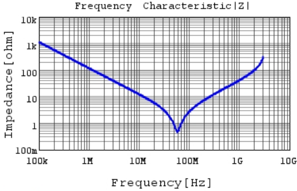
DE2E3KY152MB2BM01F |Z| DC0V, 20degC
