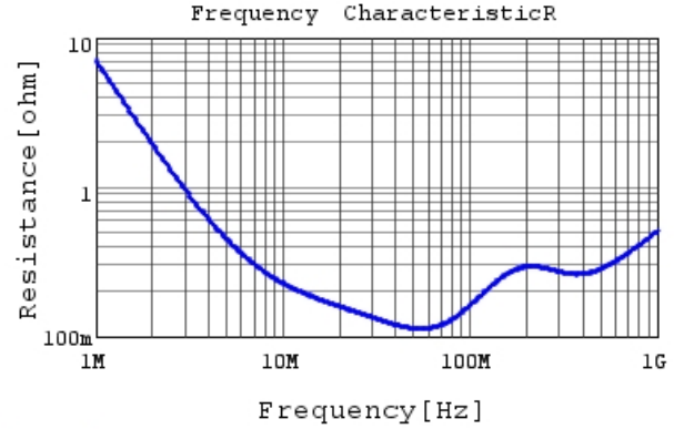
DE11XKX680JN4AC05F R DC0V, 20degC
