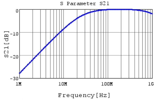
DE11XKX680JN4AC05F S21 DCOV, 20degC
