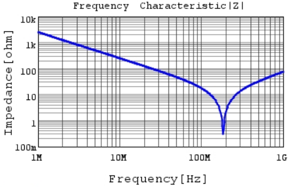
DE11XKX680JN4AC05F |Z| DC0V, 20degC
