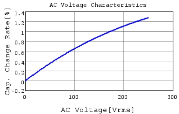
DE11XKX680JN4AC05F C-AC Voltage capchange, I
