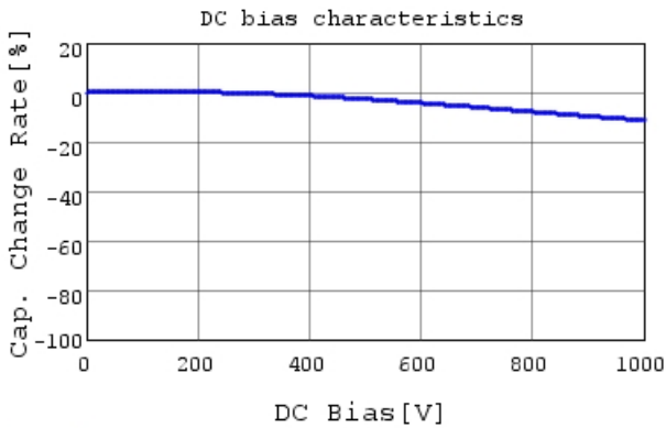
DE1B3RA151KJ4BH01F C-DC bias capchange, 20.0
