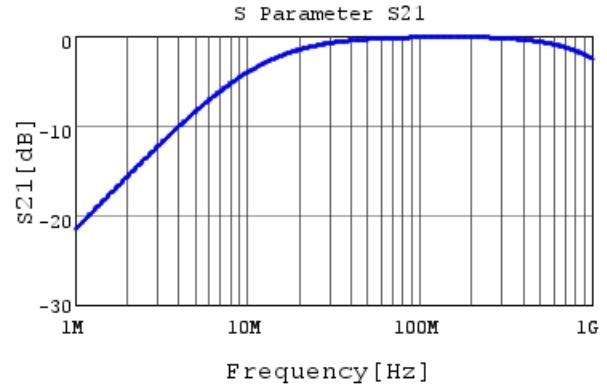
DE1B3RA151KJ4BH01F S21 DCOV, 20degC
