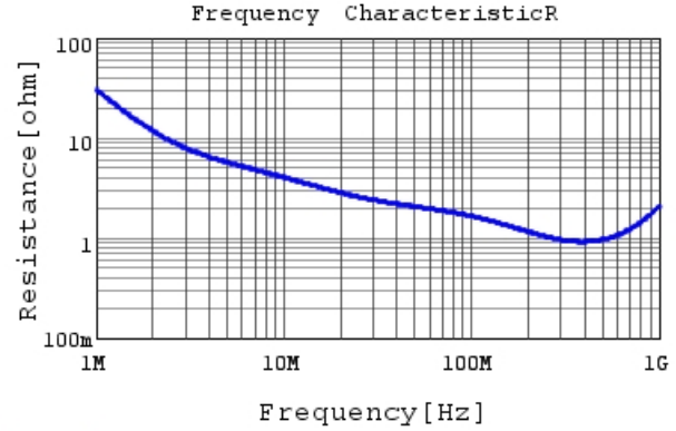
DE1B3RA151KJ4BH01F R DC0V, 20degC
