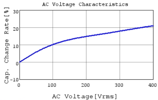
DE1B3RA151KJ4BH01F C-AC Voltage capchange, I
