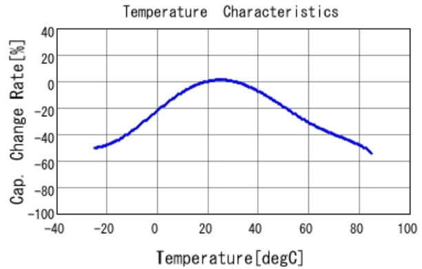
DE1E3RB102MA4BR01F C-Temp. capchange, DCOV, AC1Vrr
