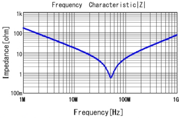
DE1E3RB102MA4BR01F |Z| DCOV, 20degC
