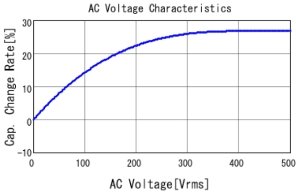
DE1E3RB102MA4BR01F C-AC Voltage capchange, DCOV, 2
