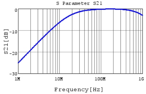
DE1B3RA101KJ4BH01F S21 DCOV, 20degC
