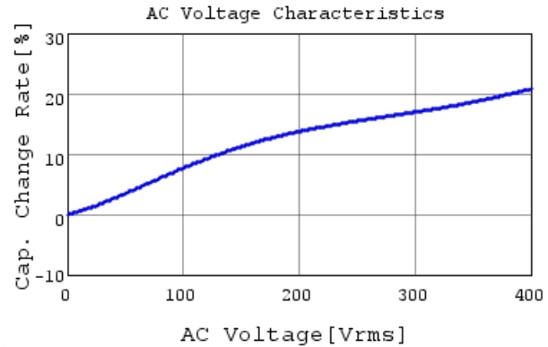
DE1B3RA101KJ4BH01F C-AC Voltage capchange, I
