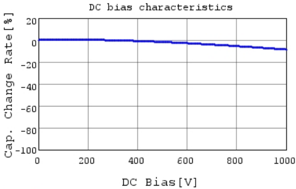
DE1B3RA101KJ4BH01F C-DC bias capchange, 20.0
