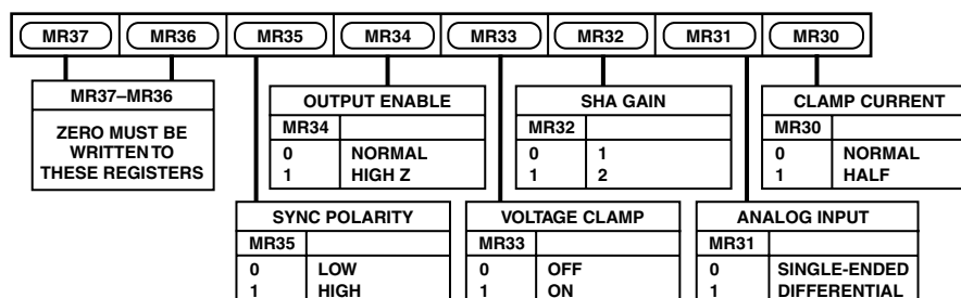
Figure 19. Mode Register 3
