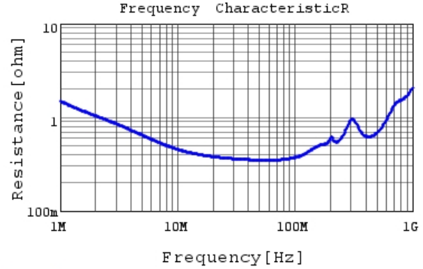
DE1E3RA332MN4AH01F R DC0V, 20degC
