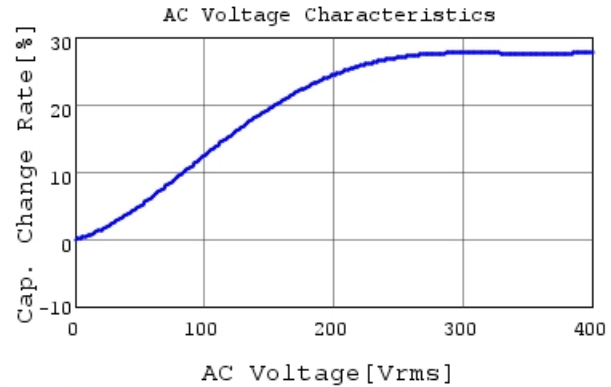
DE1E3RA332MN4AH01F C-AC Voltage capchange, I
