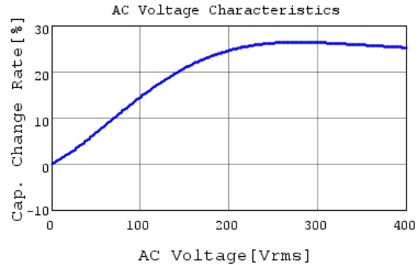
DE1E3RA152MN4AH01F C-AC Voltage capchange, I
