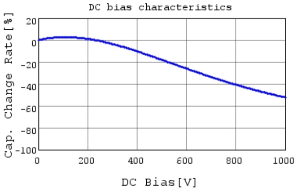
DE1E3RA152MN4AH01F C-DC bias capchange, 20.0
