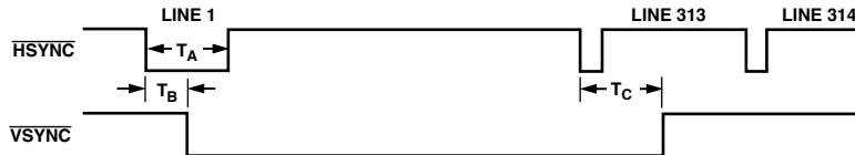
Figure 61. Timing Register 1
