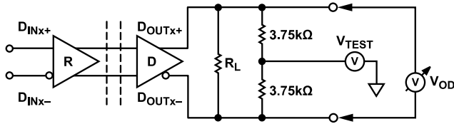
Figure 28. Driver Test Circuit
