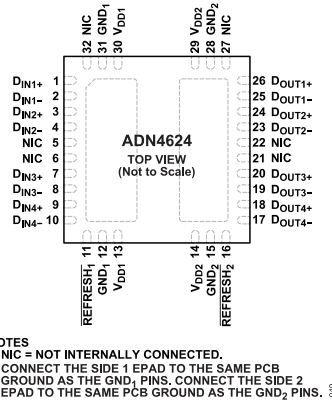
Figure 5. Pin Configuration, LFCSP
