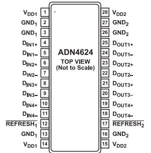
Figure 4. Pin Configuration, SOIC_W_FP
