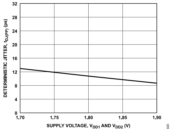
Figure 22. Deterministic Jitter, t_{DJ(PP)} vs. Supply Voltage, V_{DD1} and V_{DD2}
