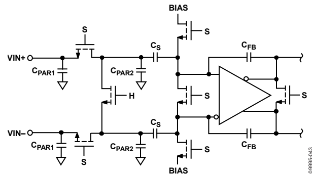
Figure 46. Switched-Capacitor Input
