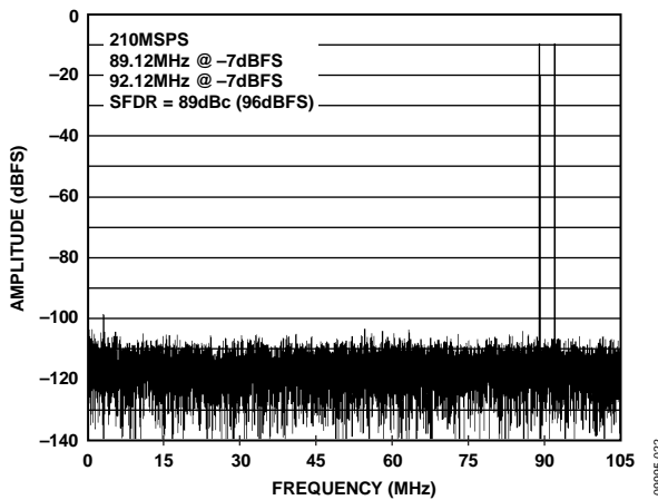
Figure 24. AD9642-210 Two-Tone FFT with f_{IN1} = 89.12 MHz, f_{IN2} = 92.12 MHz
