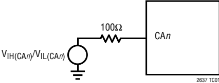
Test Circuit 1
