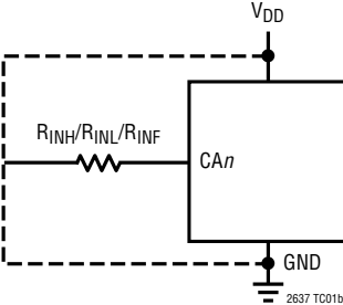
Test Circuit 2
