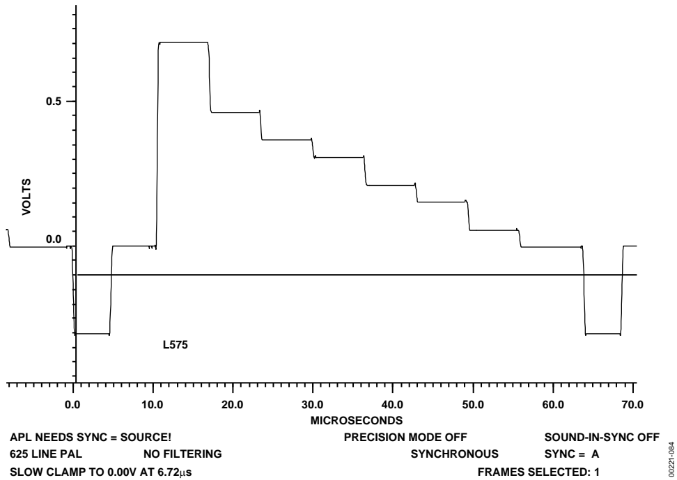
Figure 84. 100/0/75/0 PAL Color Bars Luminance
