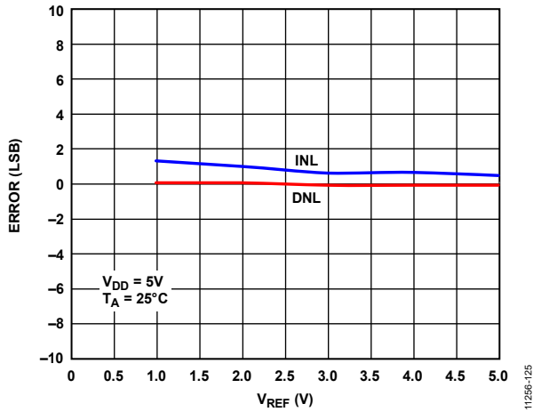
Figure 20. INL Error and DNL Error vs. V_{REF}
