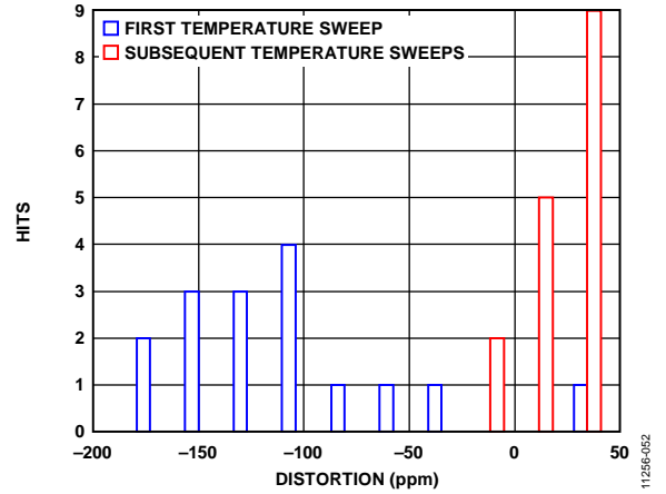
Figure 50. Thermal Hysteresis
