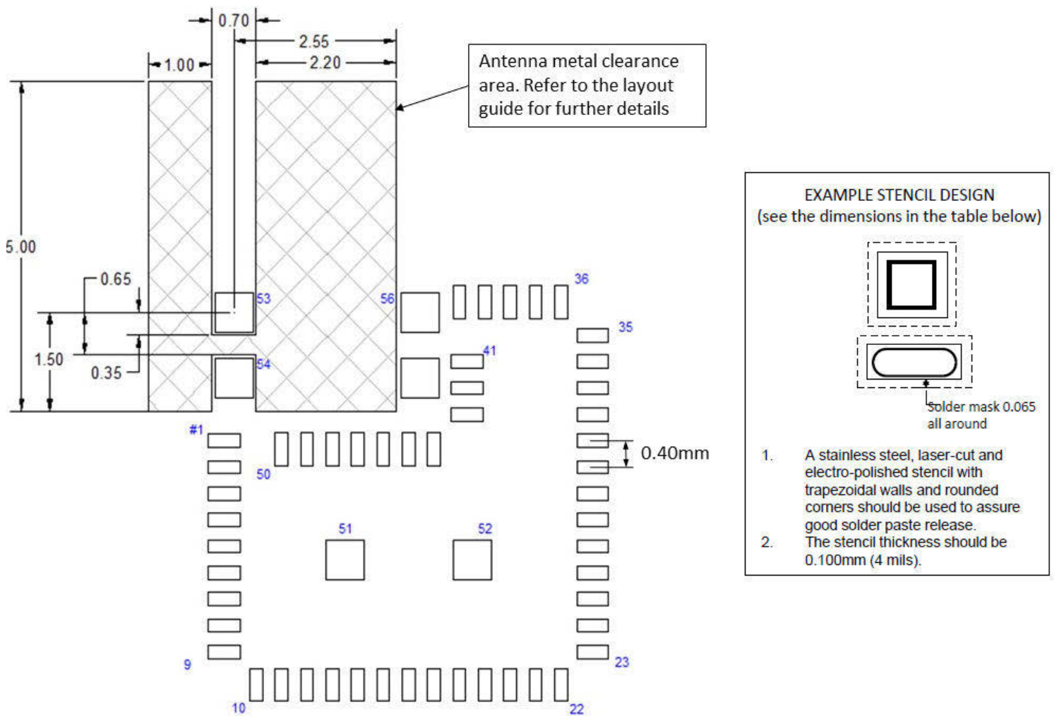
Figure 8.4. BGM11S Recommended Land Pattern
