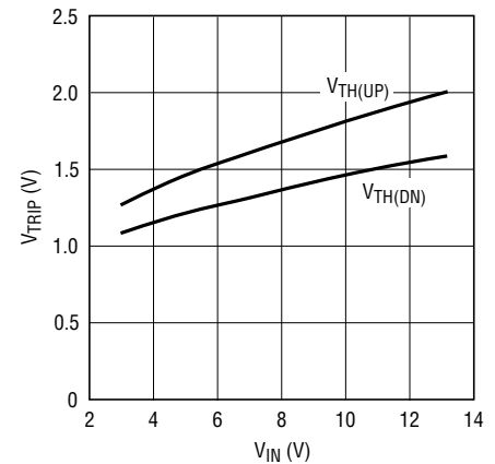
\overline{SHDN} Input Voltage Thresholds vs V_{IN}
