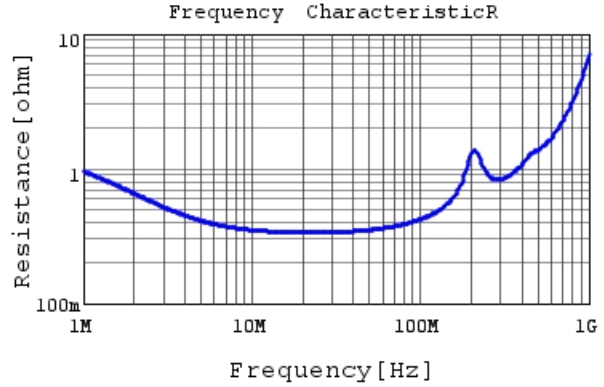
DE1E3RB472MA4BR01F R DCOV, 20degC
