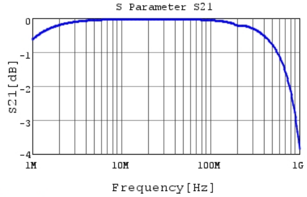
DE1E3RB472MA4BR01F S21 DCOV, 20degC
