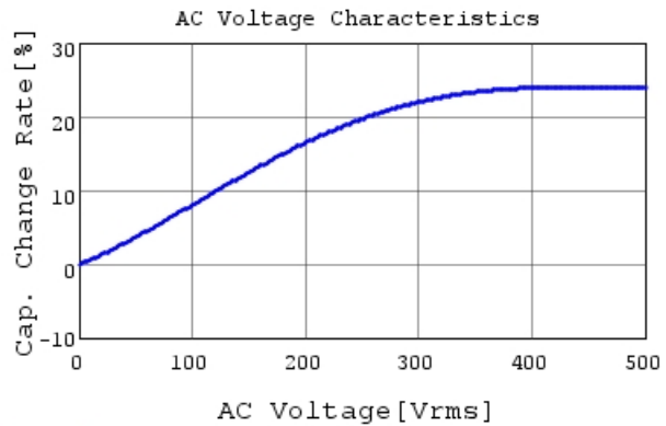
DE1E3RB472MA4BR01F C-AC Voltage capchange, I
