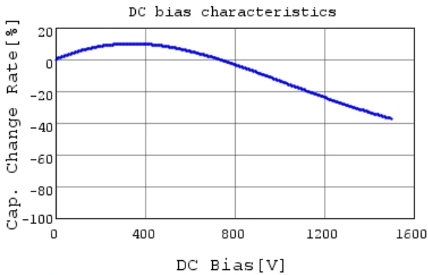
DE1E3RB472MA4BR01F C-DC bias capchange, 20.0
