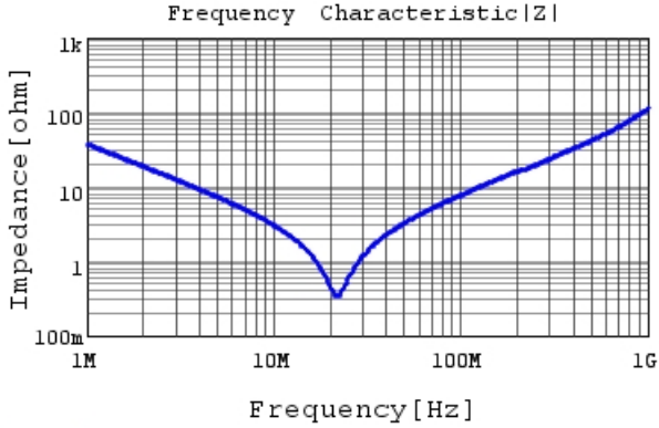
DE1E3RB472MA4BR01F |Z| DCOV, 20degC
