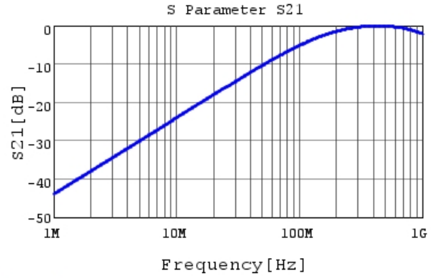
DE11XRA100KN4AN01F S21 DCOV, 20degC
