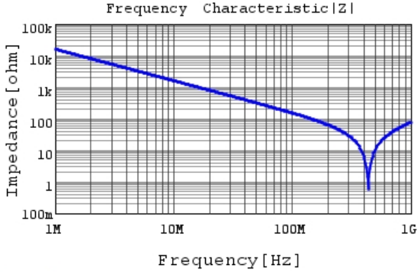
DE11XRA100KN4AN01F |Z| DCOV, 20degC
