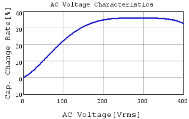
DE2E3SA102MN3AY02F C-AC Voltage capchange, I
