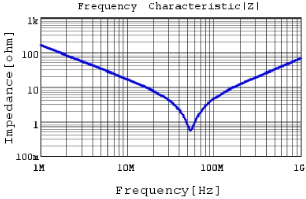
DE2E3SA102MN3AY02F |Z| DC0V, 20degC
