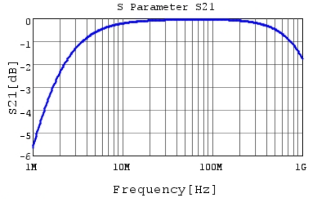
DE2E3SA102MN3AY02F S21 DCOV, 20degC
