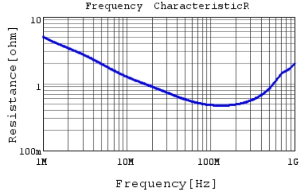
DE2E3SA102MN3AY02F R DC0V, 20degC
