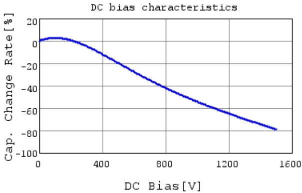
DE2E3SA102MN3AY02F C-DC bias capchange, 20.0
