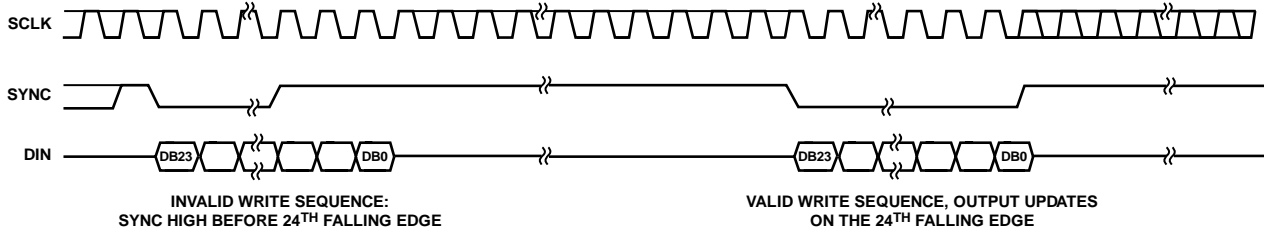
Figure 40. \overline{\text{SYNC}} Interrupt Facility
